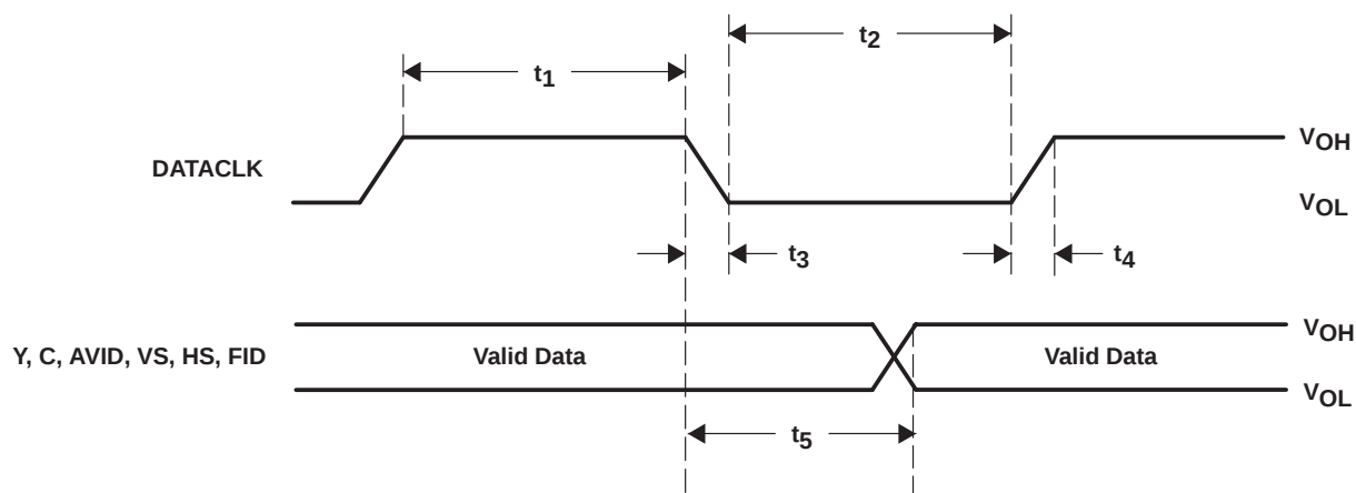
Figure 3–1. Clocks, Video Data, and Sync Timing
