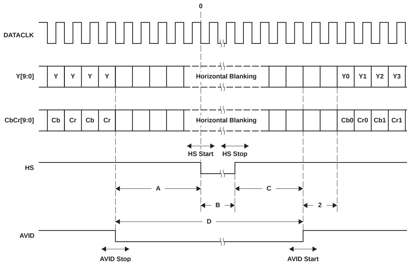
DATACLK = 1× Pixel Clock
